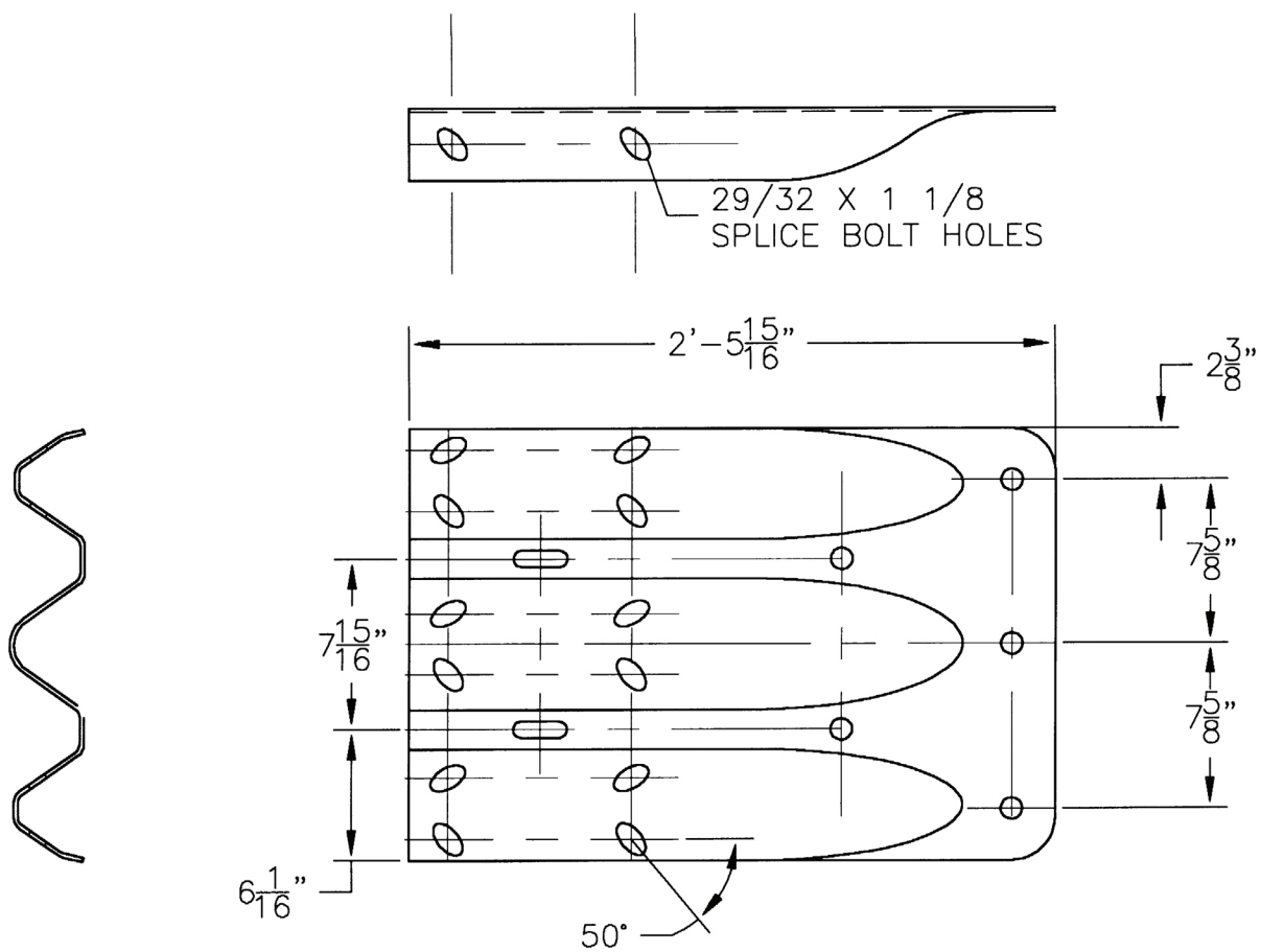
10GA/THRIE BEAM TERMINAL CONNECTOR
