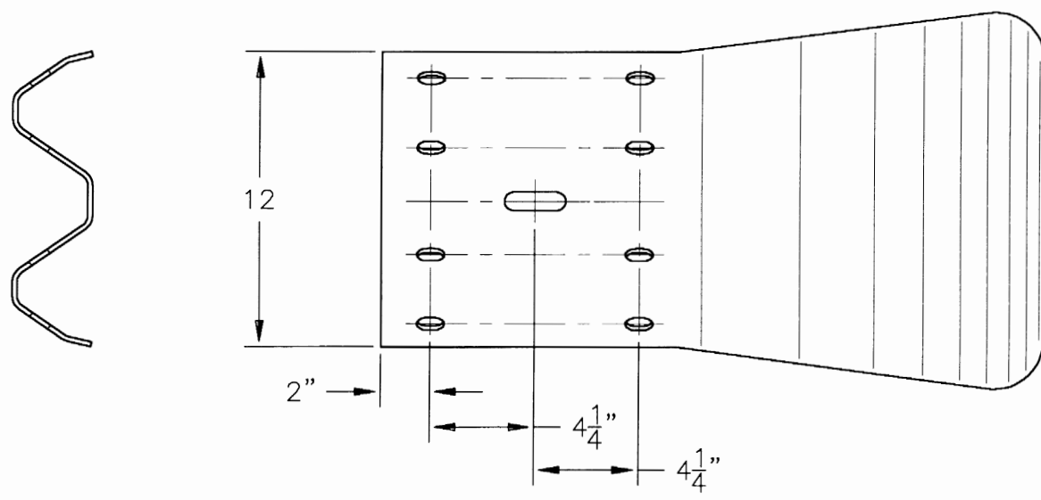
12GA/ FLARED TERMINAL
