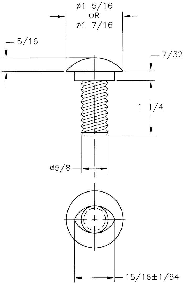
\frac{5}{8} \times 1 \frac{1}{4} SPLICE BOLT
