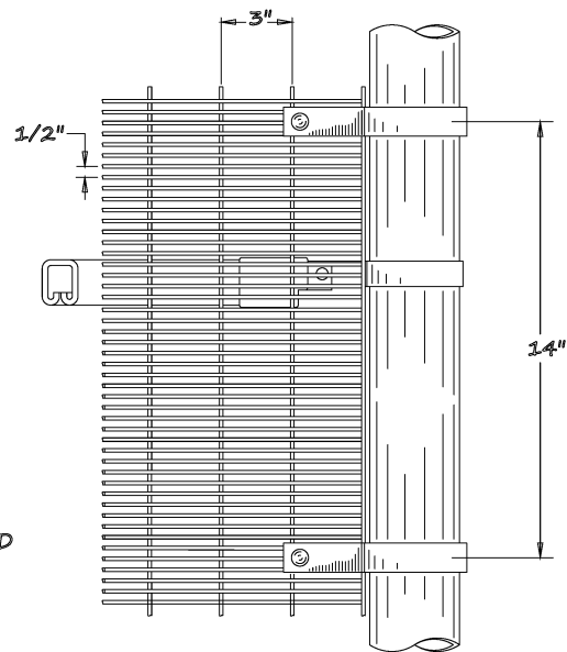
END/CORNER CONNECTION
