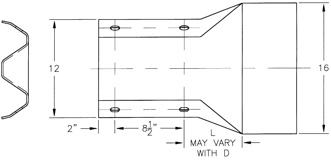
12GA/W-BEAM END SECTION (BUFFER)
